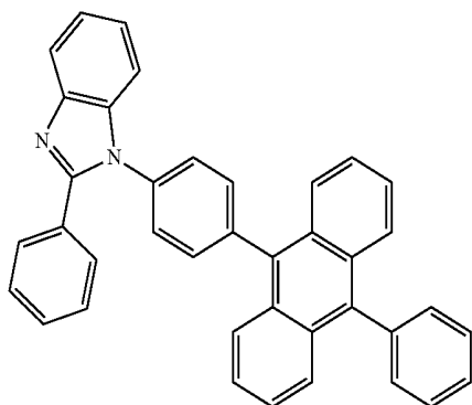
Compound ET
