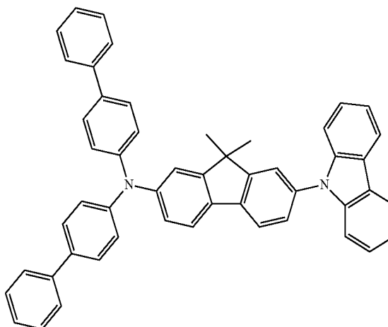
Compound HT2
