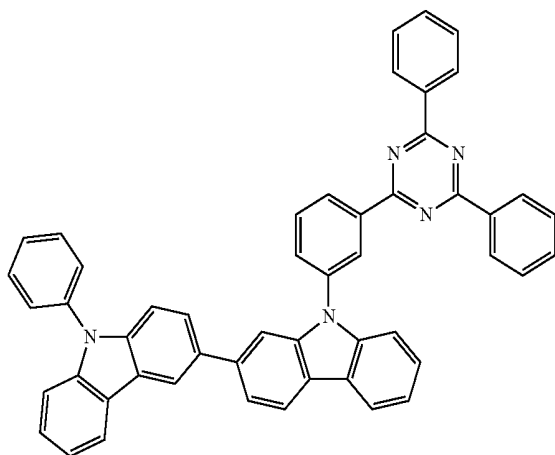
Compound ET
