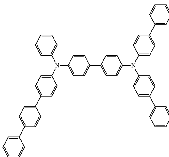
Compound HT2
